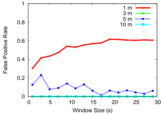
Figure 8: False positive rate for a simulated attacker who samples from the distribution of co-located devices and then uses that signal strength to impersonate one of the devices.
