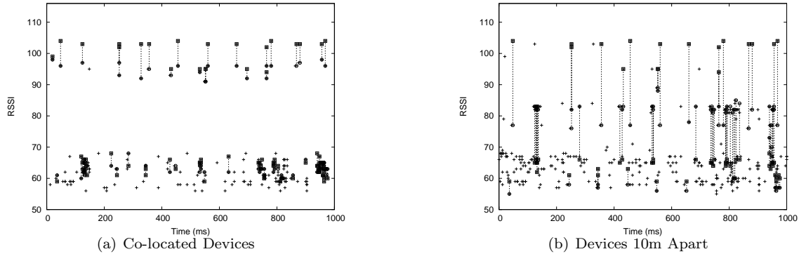
Figure 3: The received signal strength for packets heard by two devices in a 1 second period. Packets marked as “+” were received by only one laptop. Lines connect packets heard by both devices.
