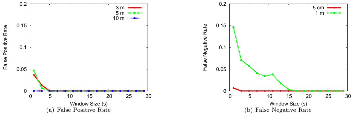
Figure 7: Co-located devices are up to 1m apart. The attackers are 3m, 5m and 10m away.
